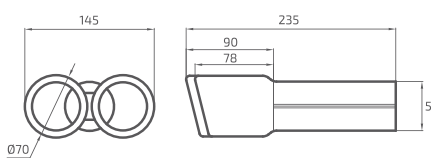
PONTEIRA REDONDA REF. 500.2-60
